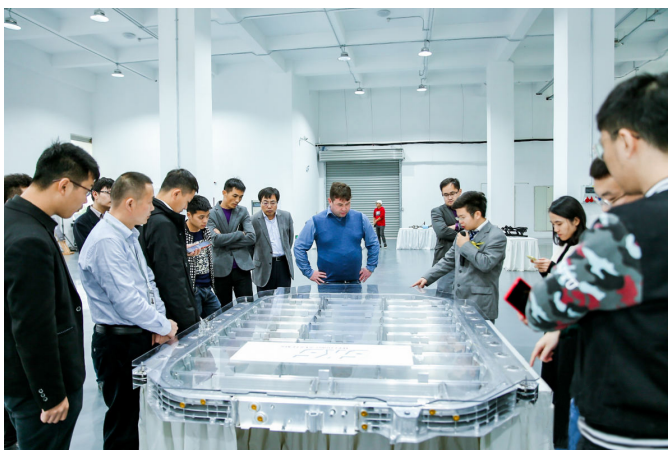
2: Battery tray welded by SKS technology of a leading vehicle manufacturer in the welding pattern exhibition
